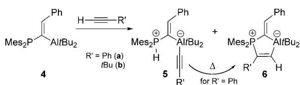
Scheme 2. Reaction of FLP 4 with terminal alkynes.
